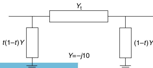
FIGURE 6.29 Pi equivalent for transformer in Problem 6.2.
