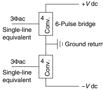
FIGURE 6.15 Single-line bipolar model.
