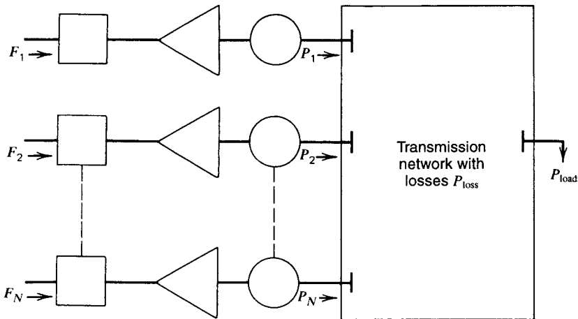
FIGURE 3.13 N_{gen} thermal units serving load through transmission network.
