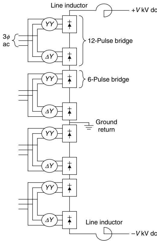
FIGURE 6.14 Converter system.
